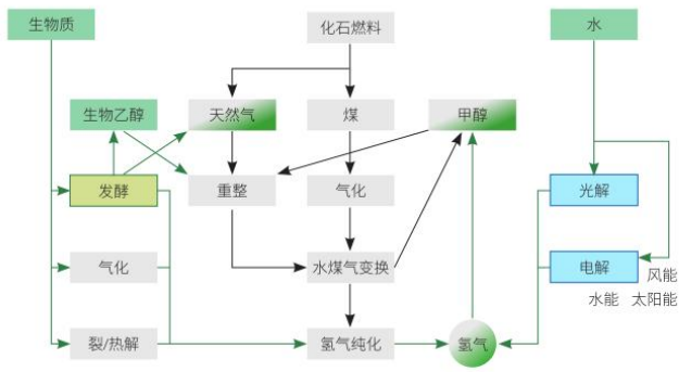
图 1 制氢工艺 Figure 1 Hydrogen production process
